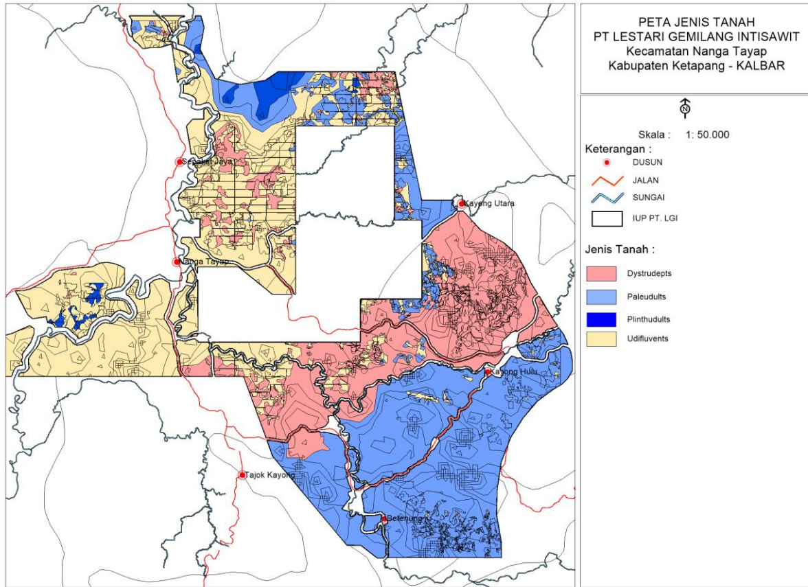
Figure 29. Map of Soil Types within concession area of PT LGI
