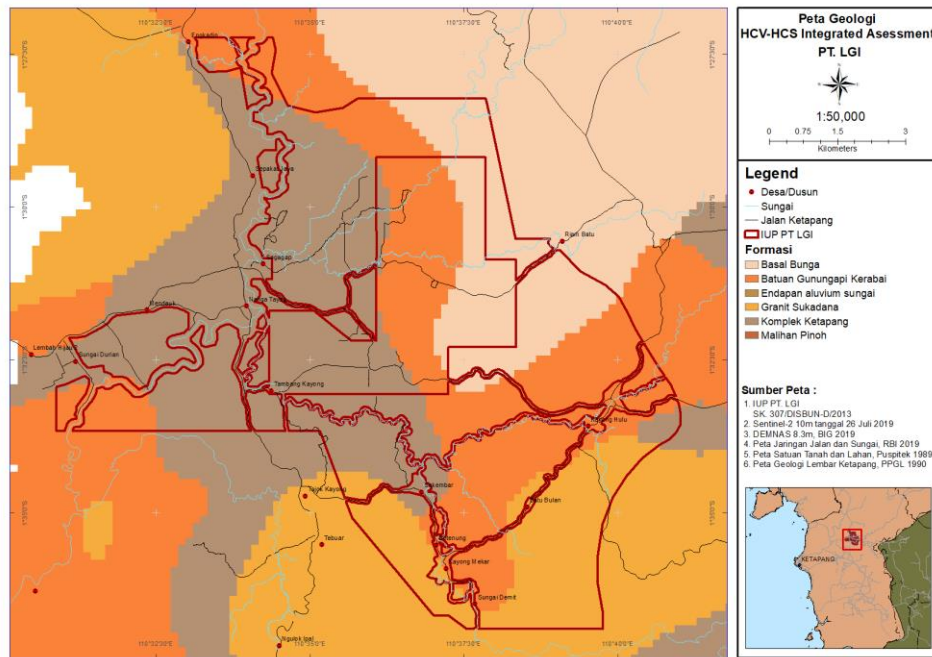
Figure 31. PT LGI Geological Map
