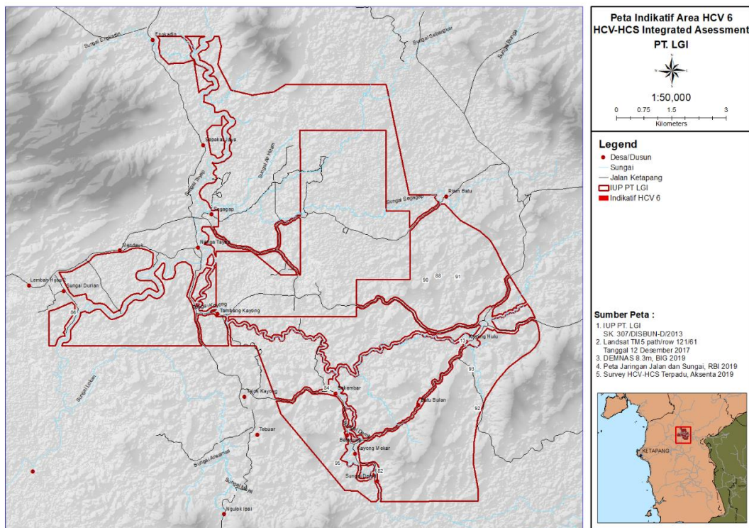
Figure 17. Map of HCV 6 Area in the area of PT LGI
