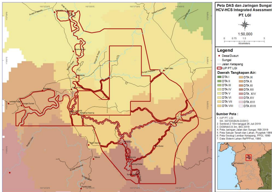
Figure 32. Watershed and River Stream at the area of PT LGI
