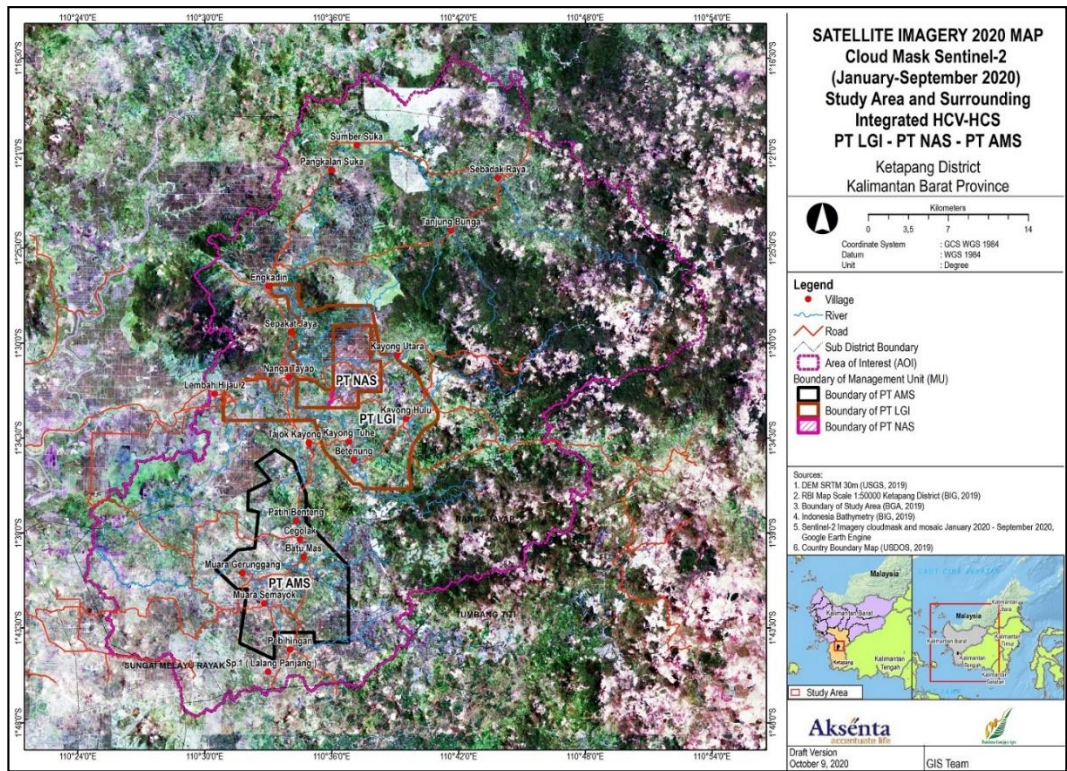
Figure 9. Sentinel-2 satellite image (January-September 2020) in the Assessment area
