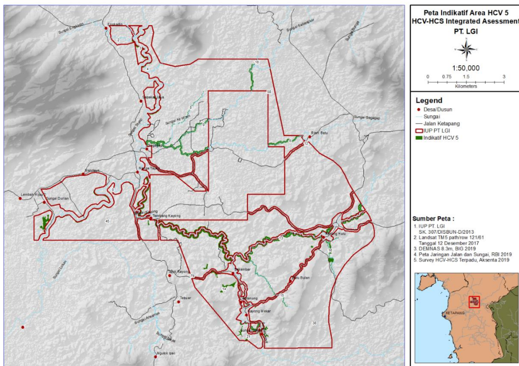
Figure 15. Map of HCV 5 Areas in the area of PT LGI
