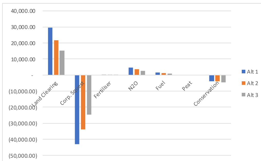
Figure 38. GHG Calculation based on land clearing alternatives
