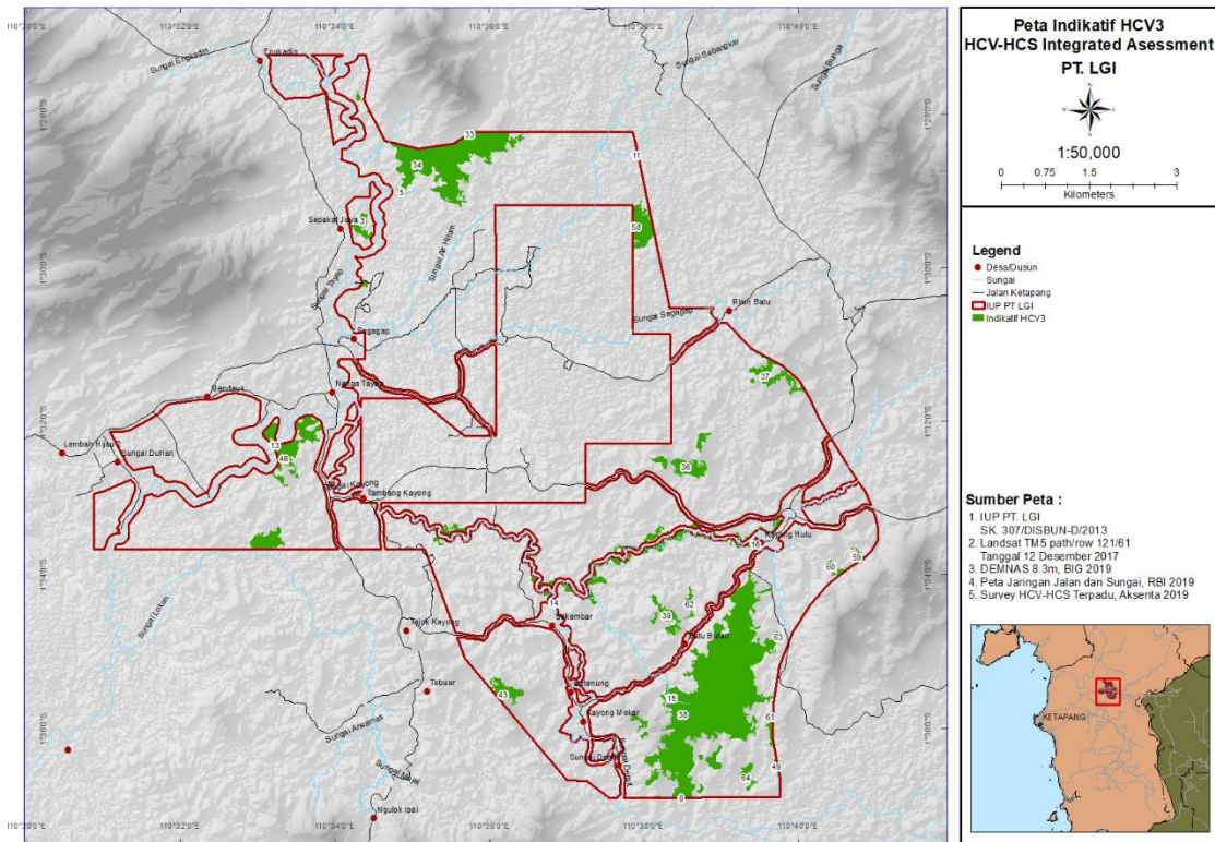
Figure 23. Map of HCV 3 in PT LGI
