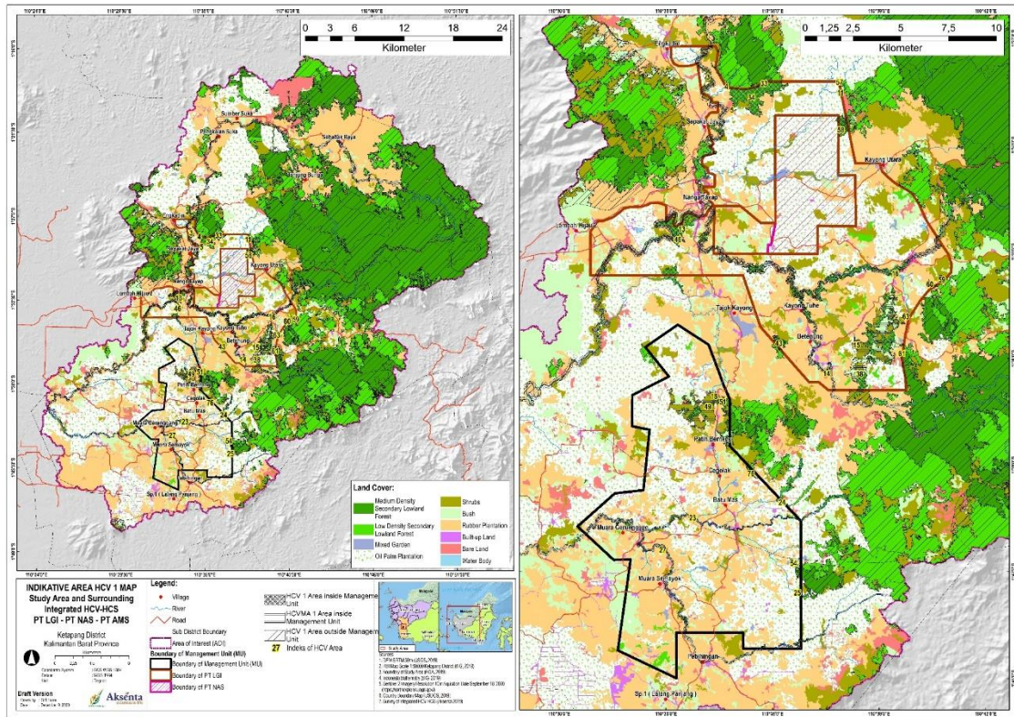
Figure 20. Map of HCV 1 Area in the Aol
