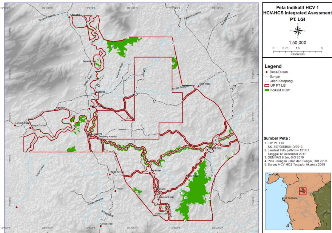
Figure 21. Map of HCV 1 Area in PT LGI
