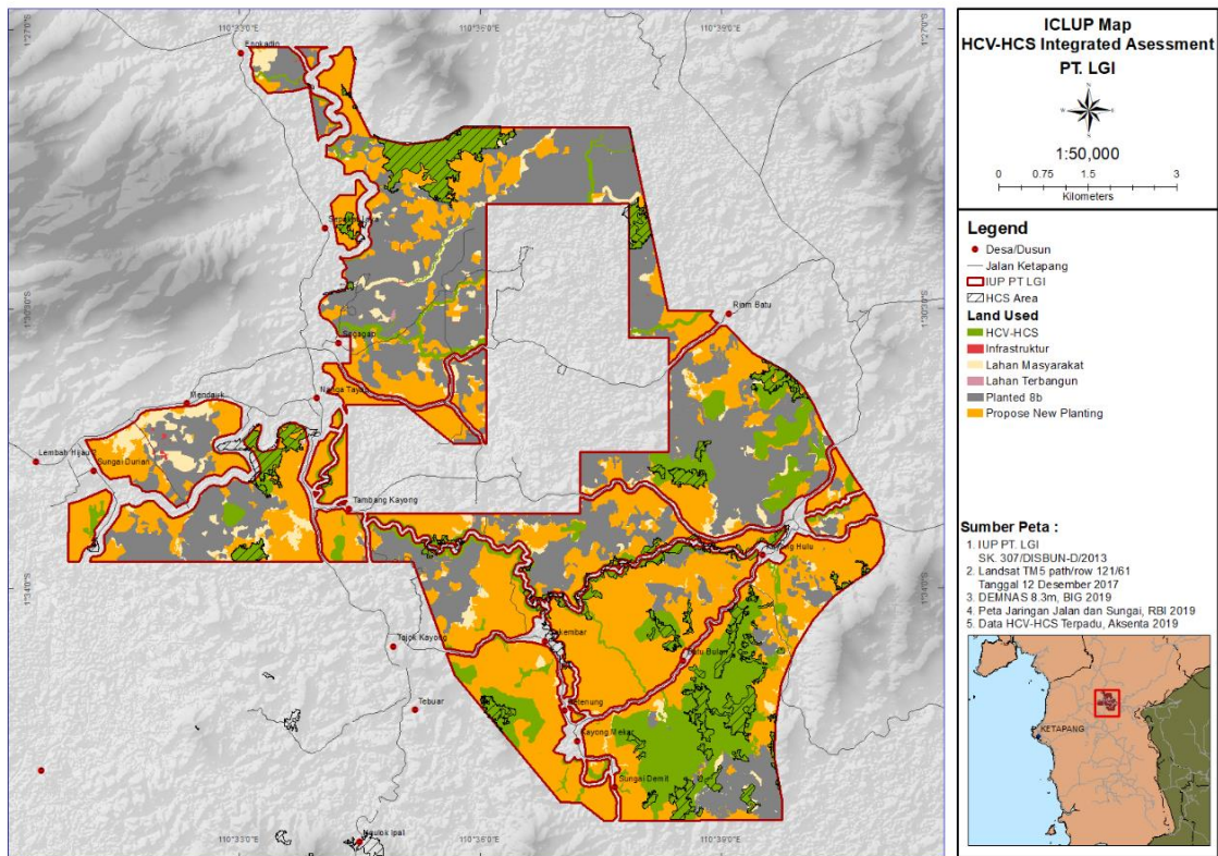
Figure 2. Indicative Conservation Land Use Plan of PT LGI
