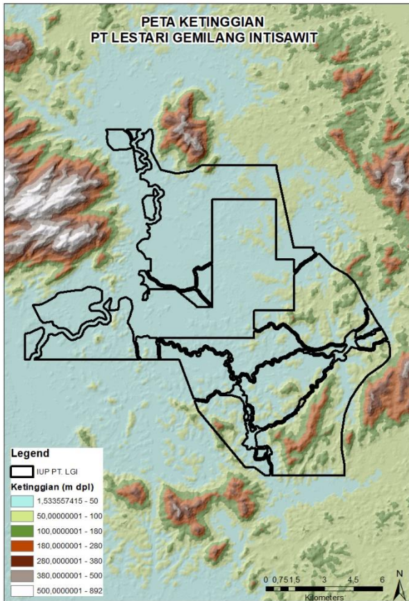
Figure 30. Left: PT LGI Topography map; Right: PT LGI Slope Class
