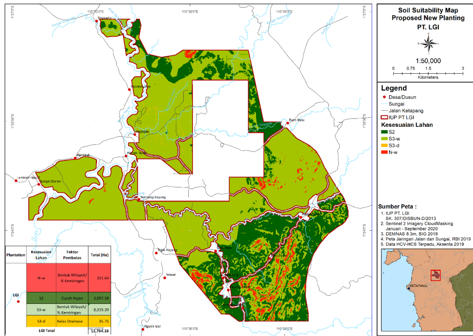
Figure 33. Map of Soil Suitability of PT LGI
