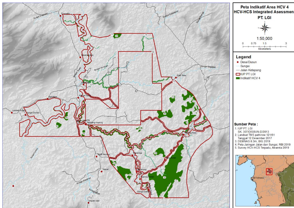
Figure 13. Map of HCV 4 in PT LGI
