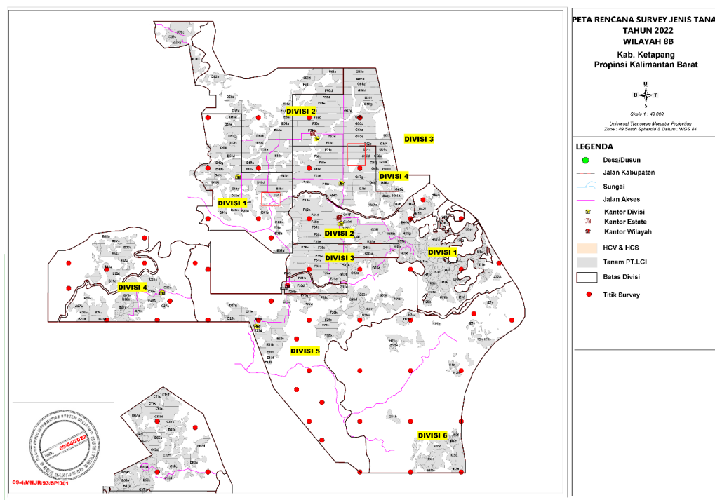
Figure 26. Map of Land Survey Plan in PT LGI
